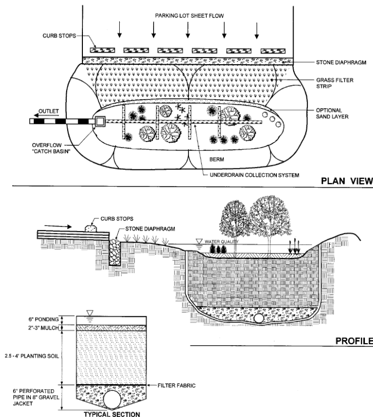
Figure 6.19 Bioretention (F-5)
